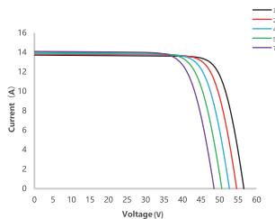
I-V Curve at Different Temperature SS8-72HD-590N
